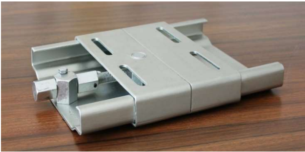
Type SMA / Dimensions (mm)
